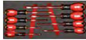
519 M 322H Code U05190927 8 PIECES 322 0,5x3x75-0,8x4x100-1x5,5x125- 1,2x6,5x150-1,6x8x175 · 322 PH 0x75- 1x100-2x125.
